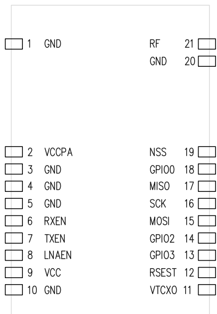
PIN define
